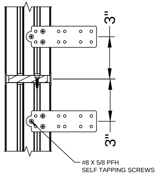
RED OAK REINFORCEMENT AT STRAP ANCHOR DETAIL AT MULLS
